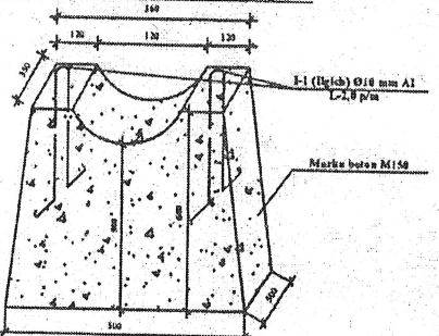
Ø102 mm gaz quvuri uchun temir beton tayanch
